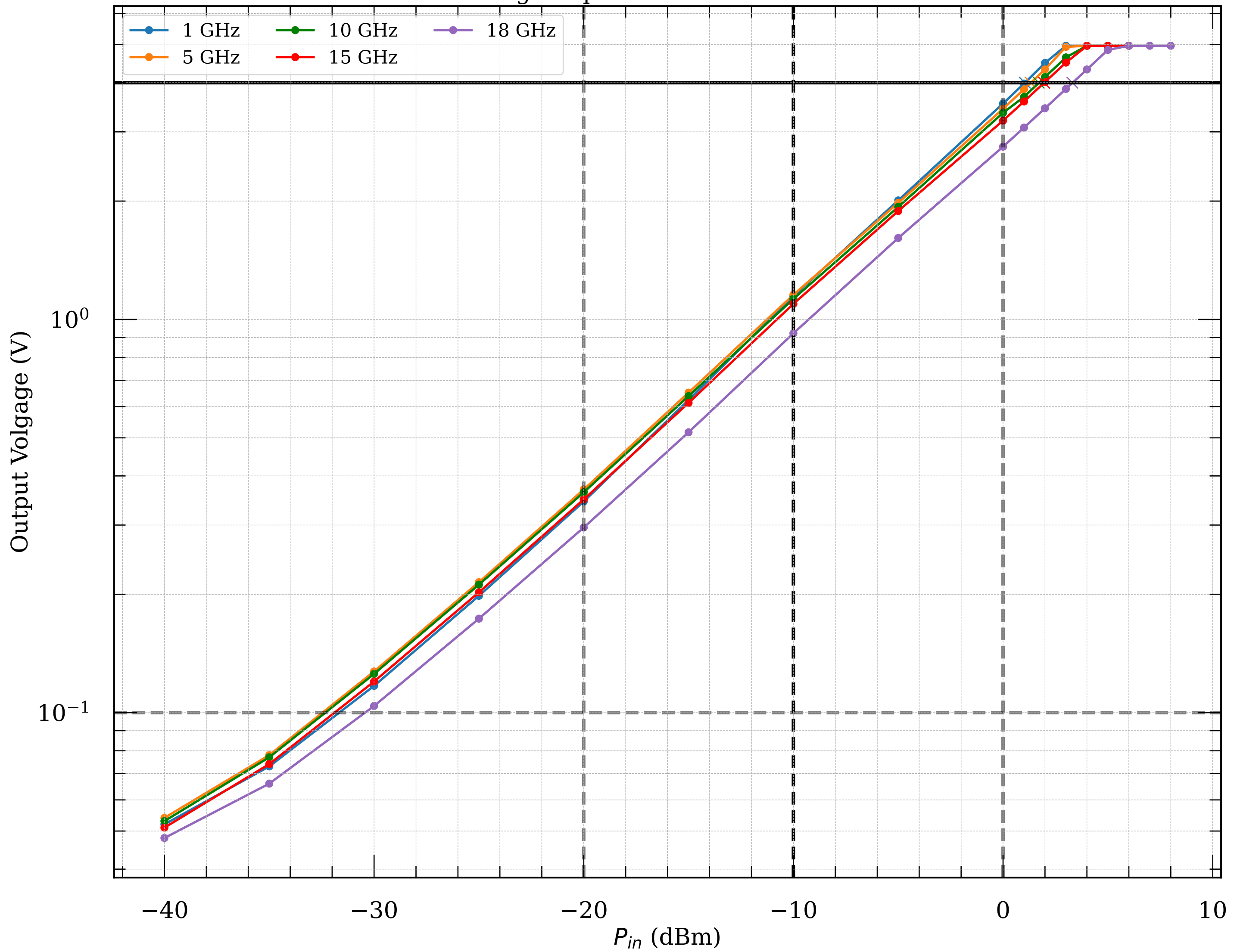
Measured voltage-to-power curve of detector module061
